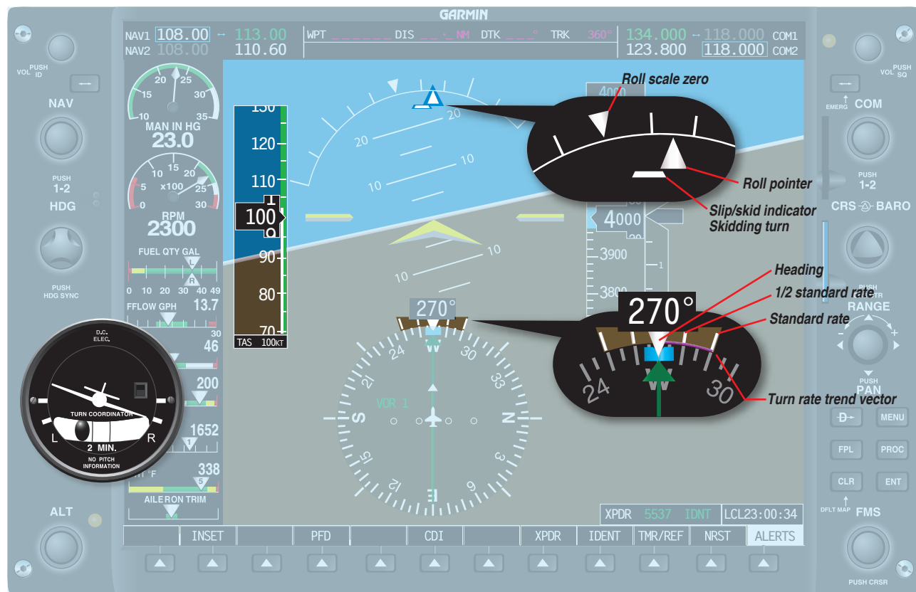
Figure 6-32. Primary bank.
