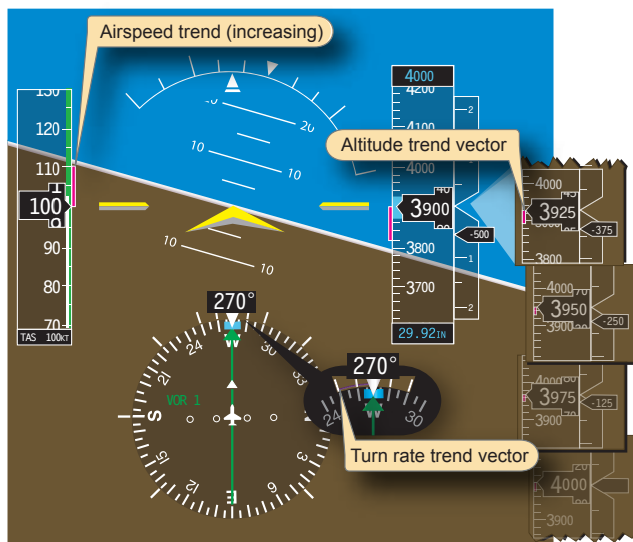
Figure 6-31. Supporting instruments.
