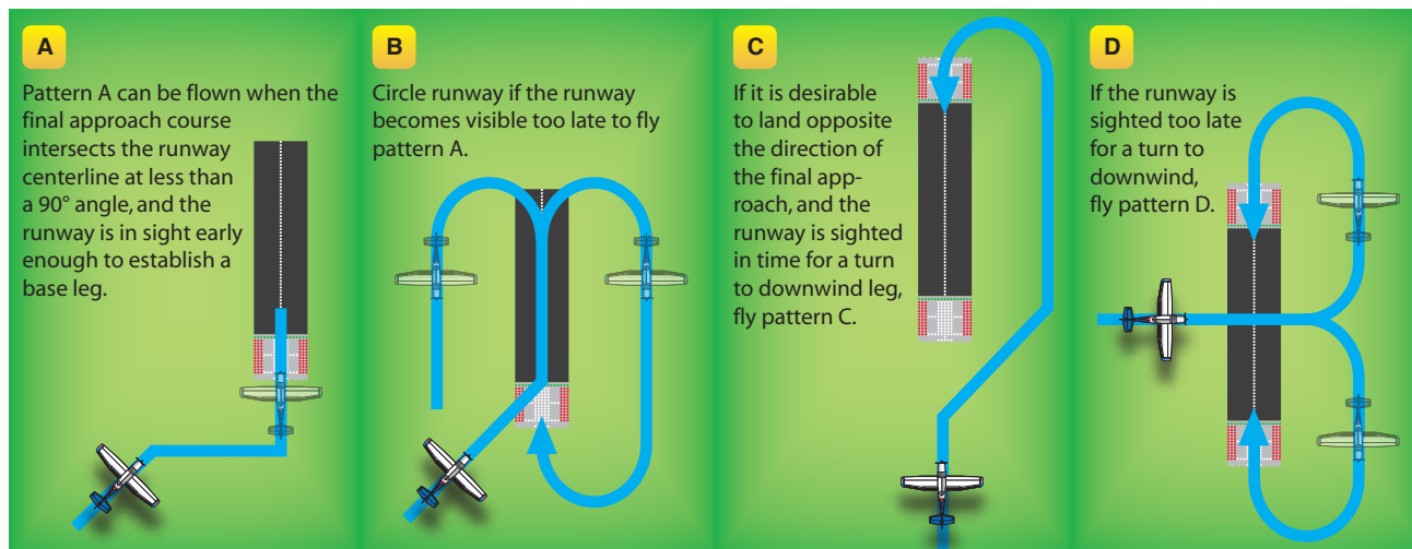
Figure 10-13. Circling approaches.
