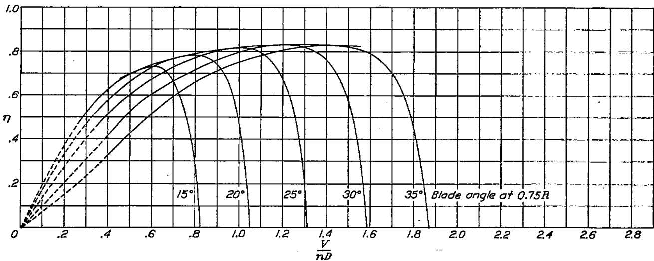
FIGURE 26.—Efficiency curves for propeller 5868-R6, R. A. F. 6 section, 4 blades.
