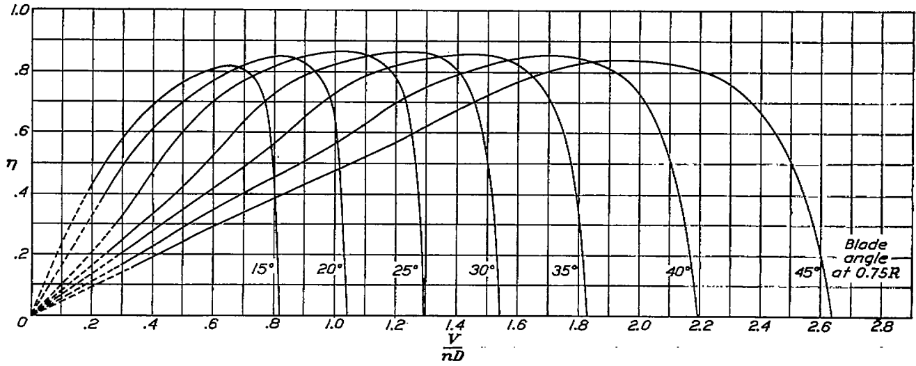
FIGURE 5.—Efficiency curves for propeller 5808-9, Clark Y section, 2 blades.
