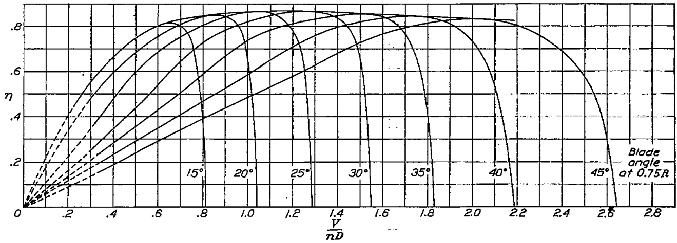
FIGURE 16.—Efficiency curves for propeller 5838-9, Clark Y section, 4 blades.
