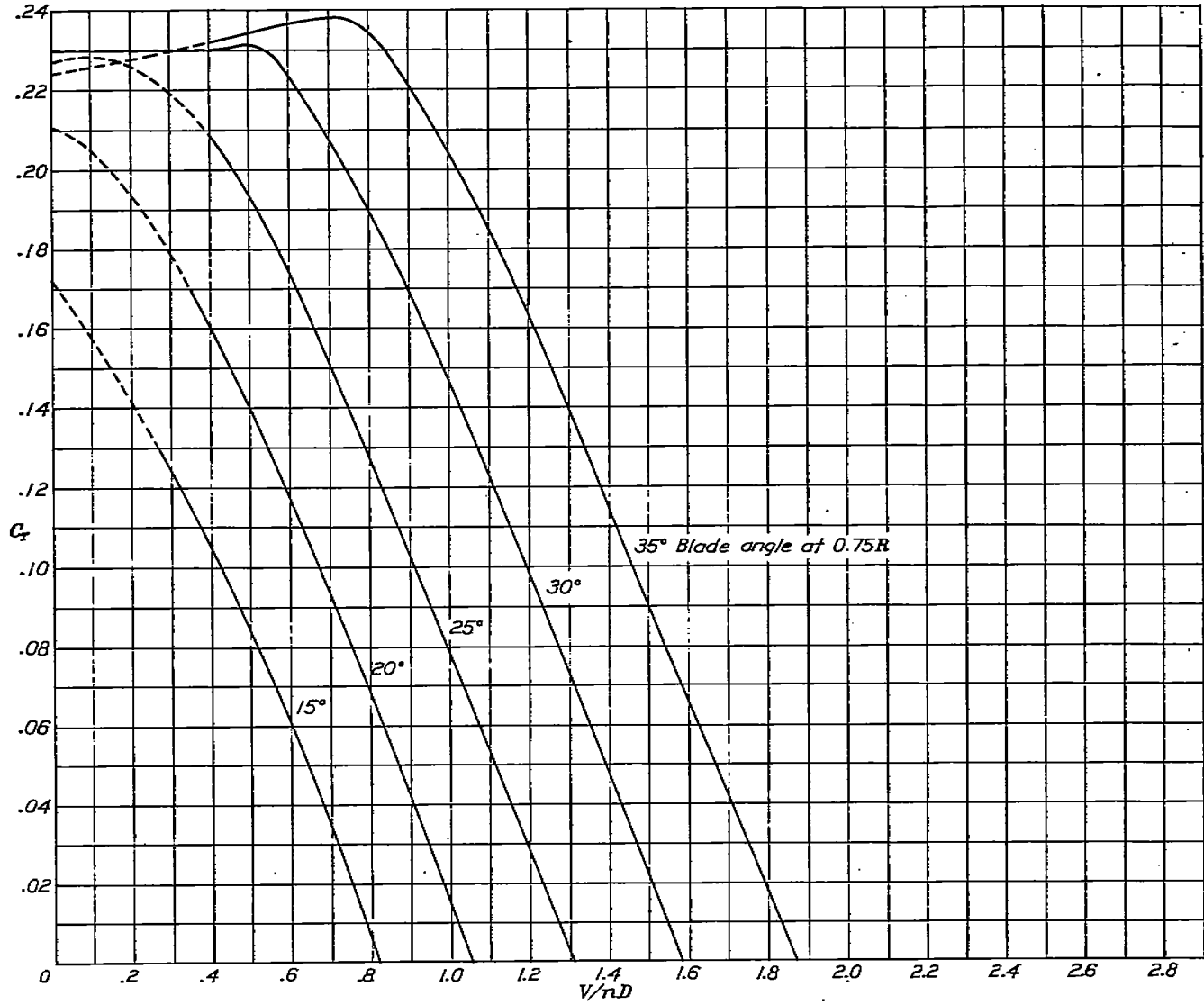
FIGURE 27.—Thrust-coefficient curves for propeller 5668-R6, R. A. F. 6 section, 4 blades.
