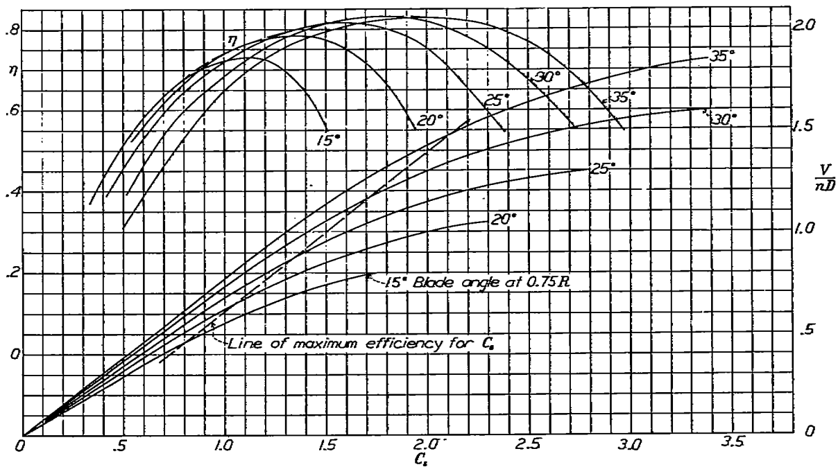
FIGURE 28.—Design chart for propeller 5668-R6, R. A. F. 6 section, 4 blades.
