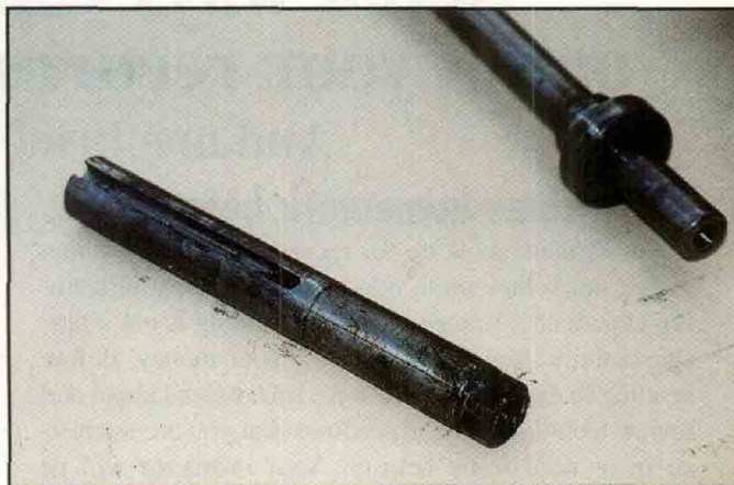
The vertical rod which mounts the bottom roller is a fairly hard piece of steel with a hole drilled in its lower end and a nut welded around it for threads. It rides up and down on the threaded rod inside the vertical tube and the slot stops it from turning. The slot is the only piece of mill work that is absolutely necessary.
